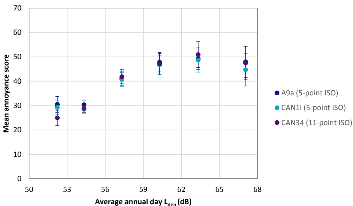
Figure 2: Plot of mean annoyance scores in SoNA 2014 survey as a function of average annual day 24hr L_{den} noise exposure
