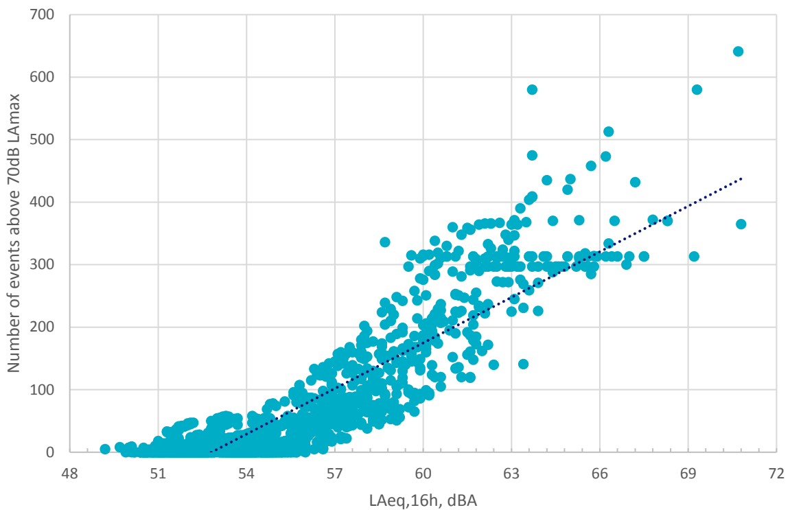
Figure 11: Relationship between N70 and L_{Aeq,16h} for resident locations surveyed
