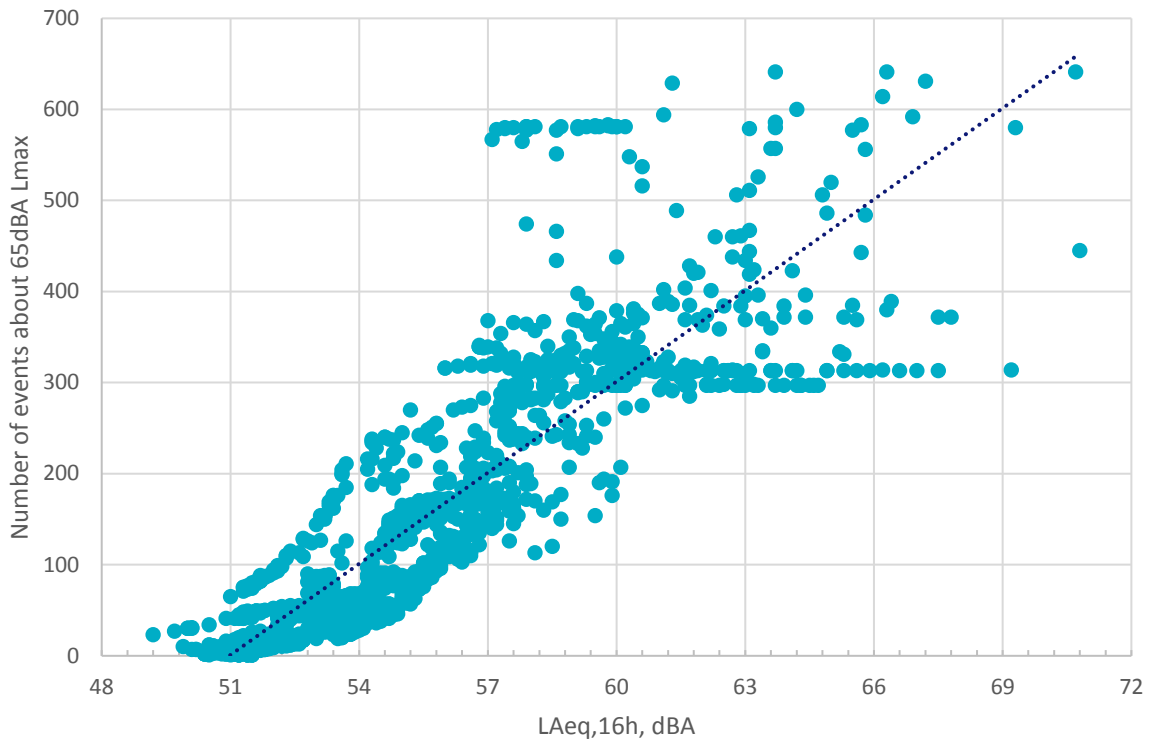
Figure 12: Relationship between N65 and LAeq,16h for resident locations surveyed
