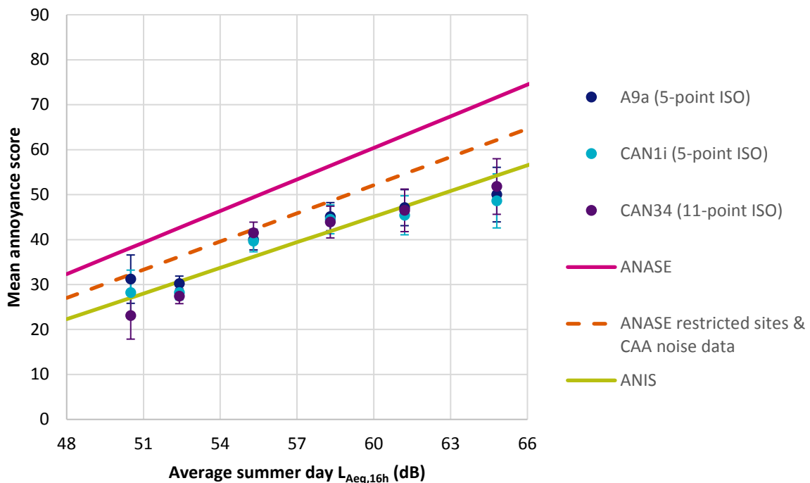
Figure 7: Comparison of mean annoyance scores for SoNA, ANASE and ANIS
